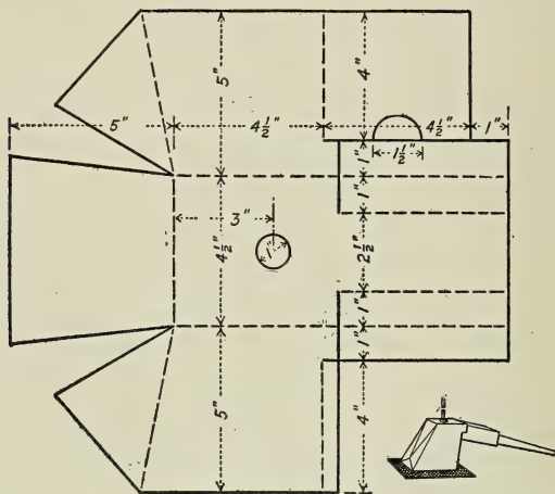
Fig. 186.—Asbestos Shield for Retort.
